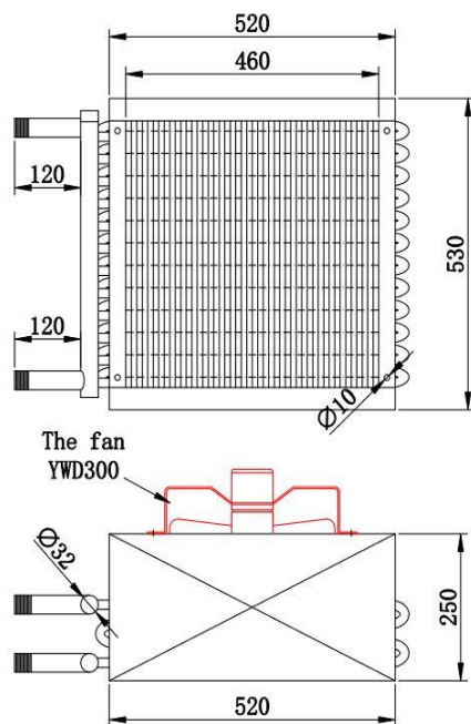
Drawing of Heater
