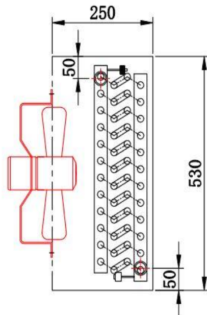
Drawing of Heater
